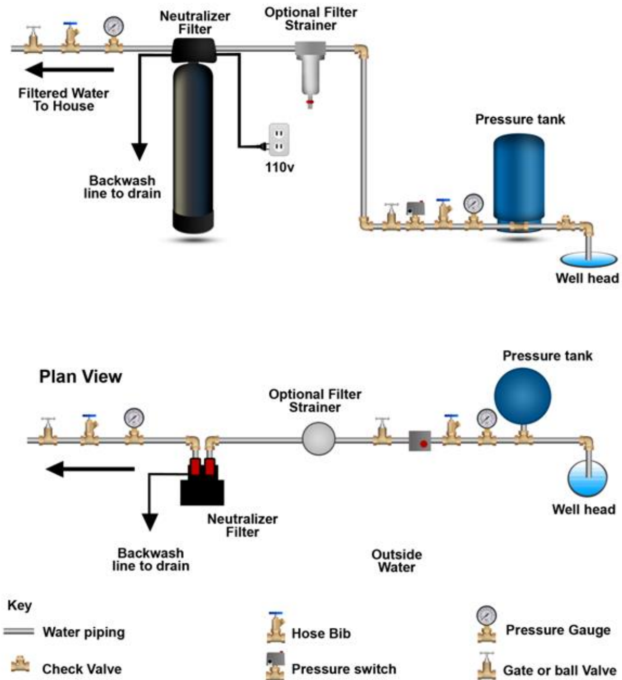
Fig 2 - Calcite Neutralizer Full Installation Diagram
